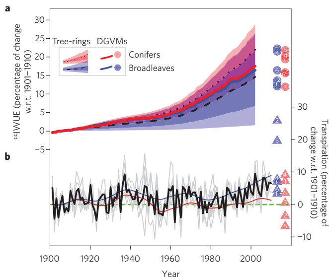
Figure 3 | Water-use efficiency and transpiration variability relative to 1901–1910. Temporal changes in the twentieth century European water balance. a , {}^c\text{iWUE} upper and lower deciles (light shaded), the 22nd and 78th percentiles (dark shaded), and median estimates (dashed) for the broadleaf and conifer sites until 2002. Ensemble means for the DGVM modelled {}^c\text{iWUE} changes for PFTs (solid lines) together with decadal mean values around 2002 (circles: 1 = CLM4CN; 2 = LPJ; 3 = LPJ-GUESS; 4 = SDGVM; 5 = TRIFFID; 6 = ORCHIDEE. b , Changes in transpiration for the European tree PFTs for the six ensemble members (grey), their mean (black), and for the smoothed broadleaf (blue) and coniferous evergreen (red) ensemble means. Coloured triangles as in a for 2001–2010.
